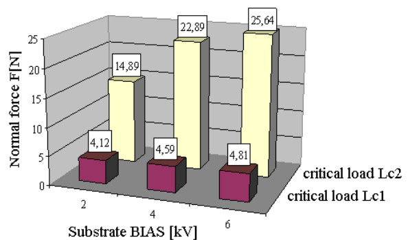
Fig. 7. Changes in the critical load of adhesion with substrate BIAS for Cr doped Cr-CrN-DLC coatings
