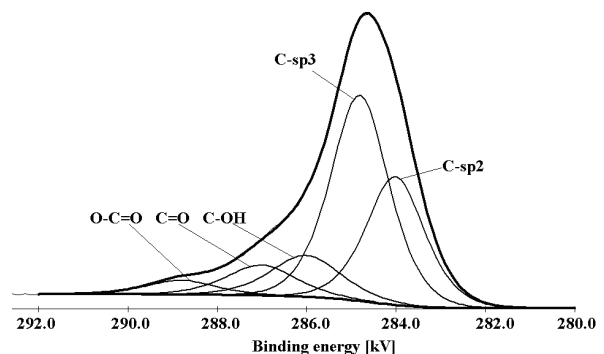
Fig. 5. C1s peaks of XPS spectrum of DLC coating doped with chromium
